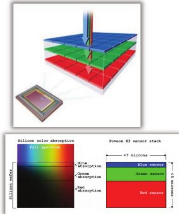
Foveon X3
